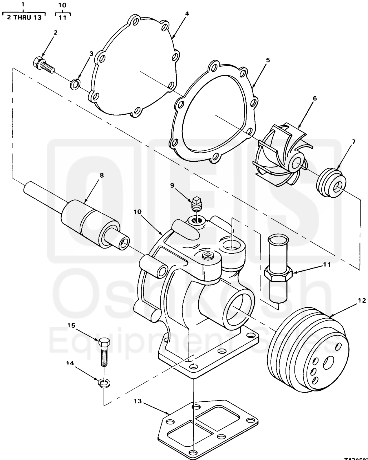
FIGURE 47. WATER PUMP.
